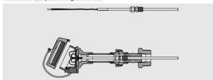
Fixed connection (compression fitting) to the furnace
