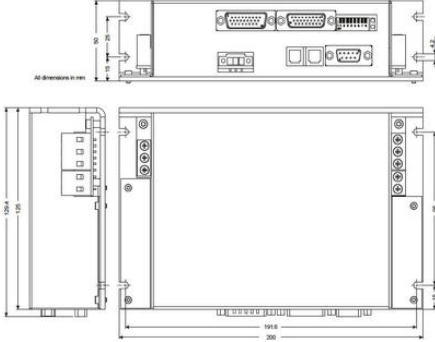
IDM3000 drives dimensions
