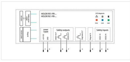
HOLDX_R_1 standalone 8-pin pigtail without EDM function
