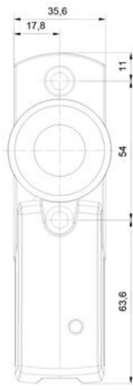
Magnet unit
