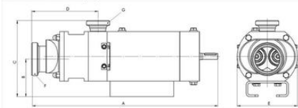
Mäz HYGHSPIN Extended (l) axial (mm)
