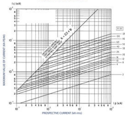
Cut-off characteristics
