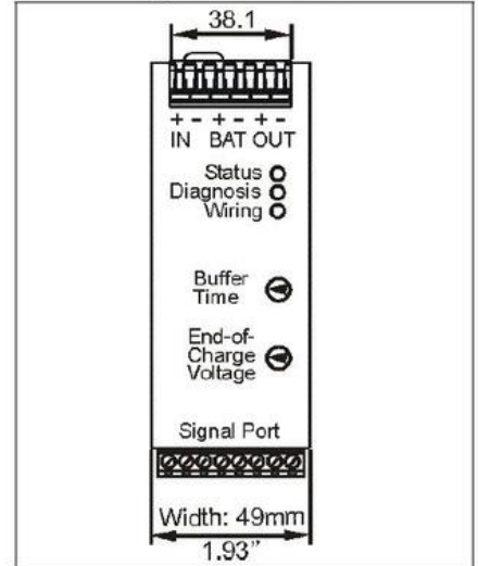
Fig. 24-2 Front view
