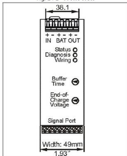
Fig. 24-2 Front view
